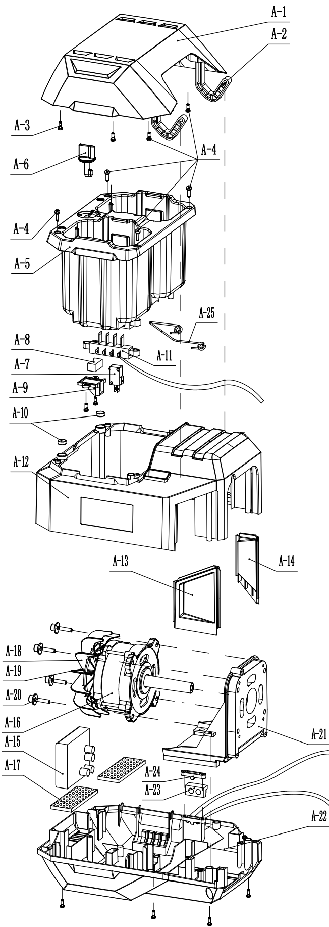
A 58V DC motor set
